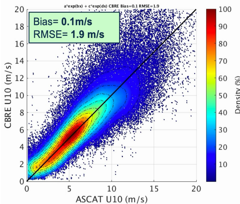
Figure 3 – TechDemoSat-1, NOC CBRE wind retrieval validation
